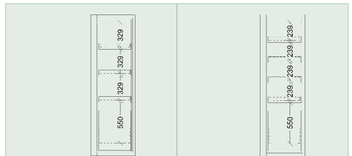
SiS Type 90 / 600 VS4-ES, Art. No. B80-2588-B, RAL 7035, incl. 4 pull-out shelves and 1 disposal compartment
