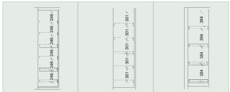
SIS Typ 90 / 600 VS6, Article No. B80-2570-B, RAL 7035, incl. 6 pull-out shelves
